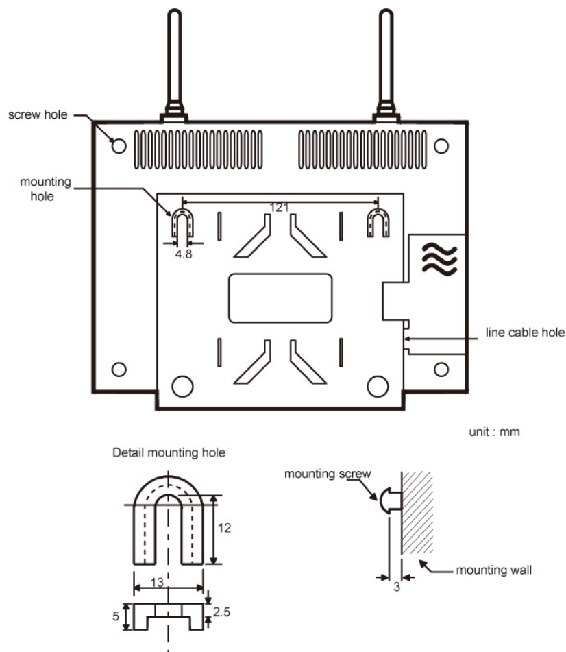
Figure 3.4.2.1-1 Back side of GDC-600BE
