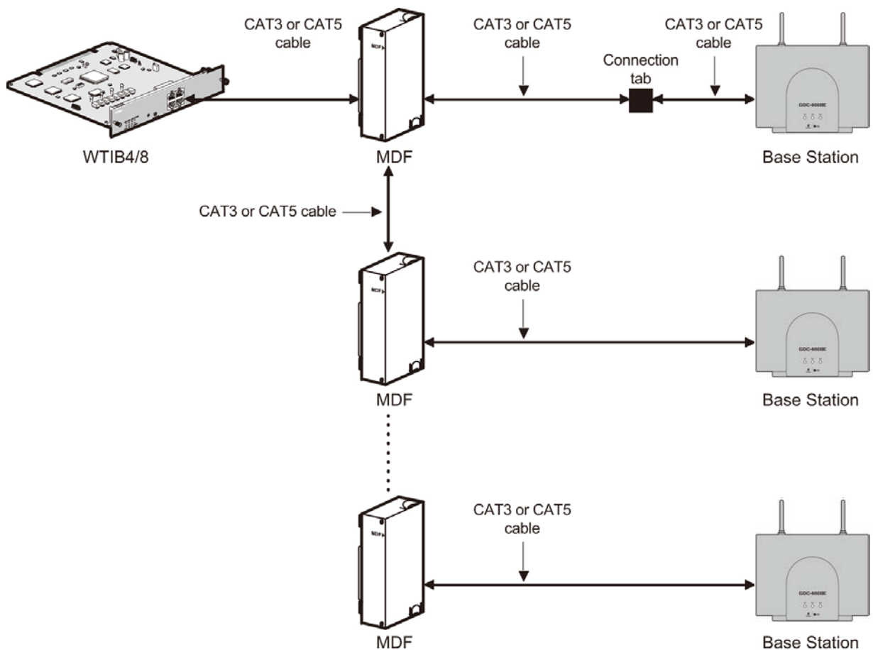
Figure 3.5-3 Wiring with MDF and connection tab between WTIB4/8 and Base Station
