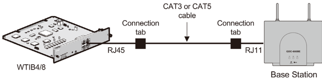
Figure 3.5-2 Wiring with connection tab between WTIB4/8 and Base Station
